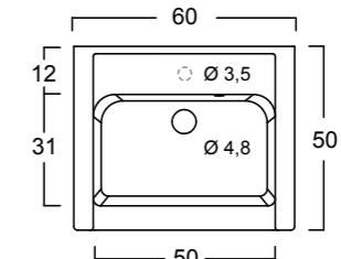
Cod. 965
