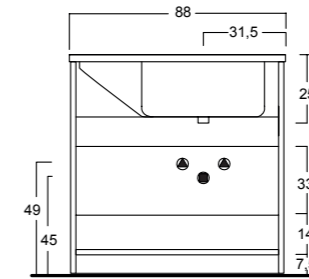
COD.22Z85DX
