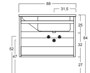
COD.22C285DX
