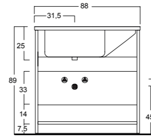
COD.22Z85SX
