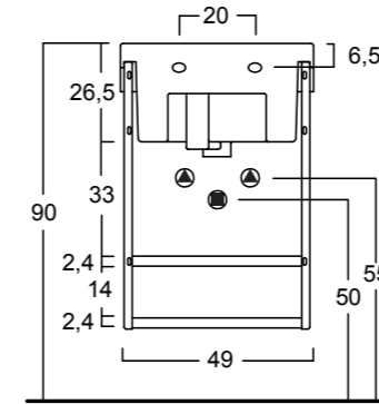
Cod. 21ML50 - 955
