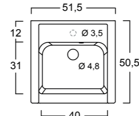
Cod. 955
