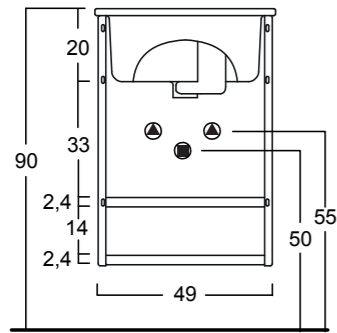
Cod. 21ML50 - 855
